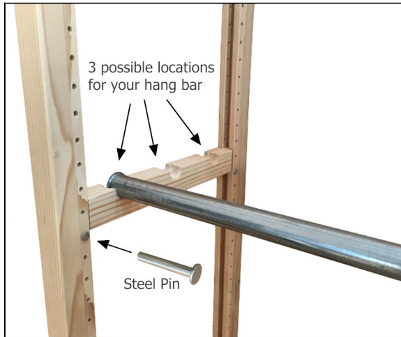
Insert steel pins to desired height of wood support rail
